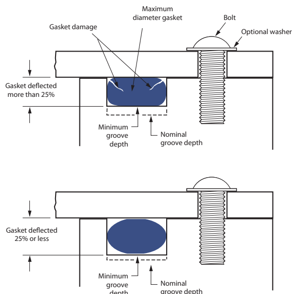
Figure 3-20 Section B-B from Figure 3-19 – Worst Case Maximum Deflection (Maximum gasket diameter, minimum groove depth)
