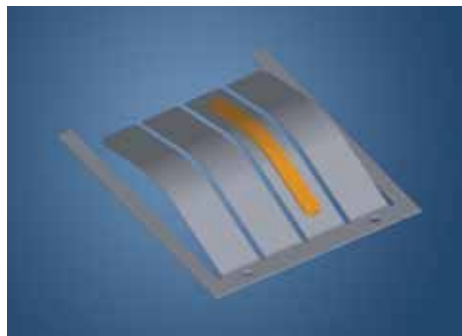
CHO-Seal 1273 overmolded on metal stampings provide discrete grounding points.
