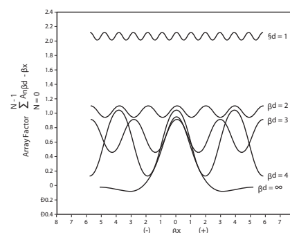
Figure 3-12. Array Factor vs. Spacing
