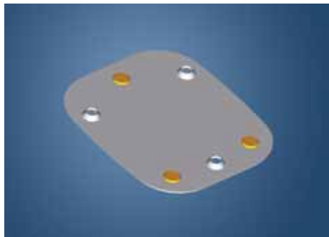
CHO-Seal 1273 overmolded on metal stampings provide discrete grounding points.
