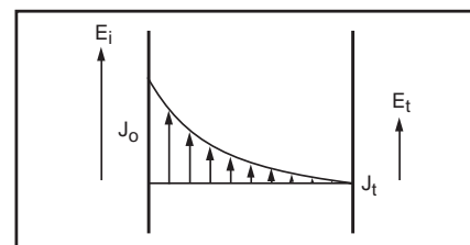
Figure 1-2 Variation of Current Density with Thickness for Electrically Thick Walls
