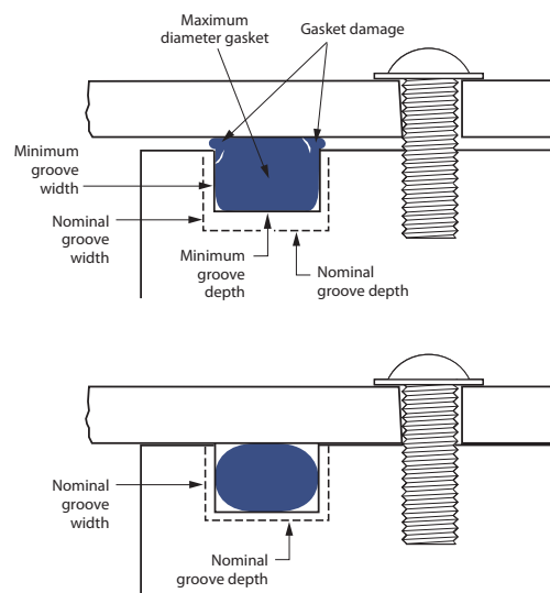
Figure 3-21 Section B-B from Figure 3-19 – Worst Case Maximum Groove Fill (Maximum gasket diameter in minimum groove depth and width)
