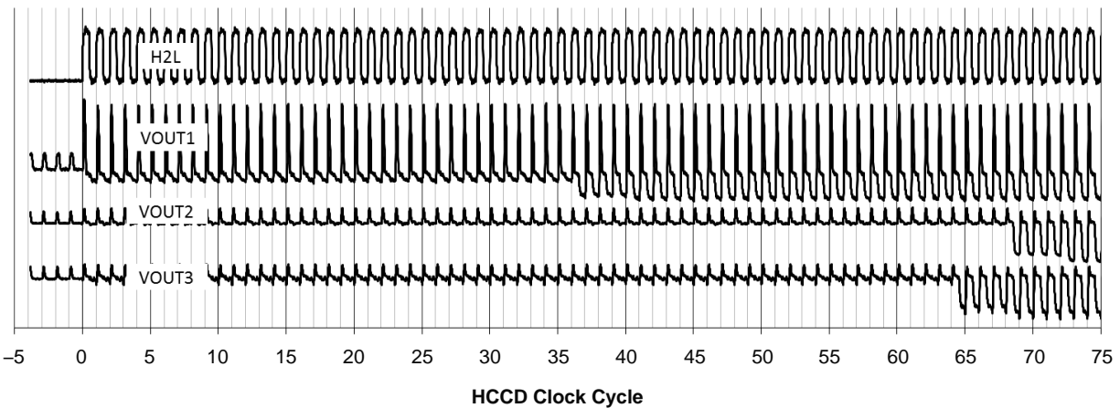
Figure 22. The Video Output Waveforms at the Start of Each Line with No Horizontal Charge Binning, for 1, 2, or 4-Output Mode
