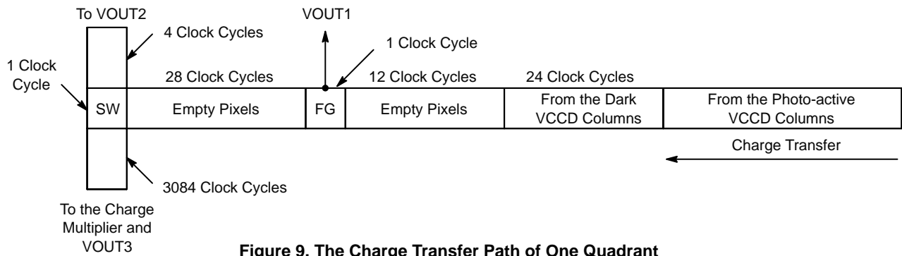
Figure 9. The Charge Transfer Path of One Quadrant
