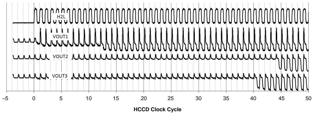
Figure 27. The Video Output Waveforms at the Start of Each Line with 3x Horizontal Charge Binning. This is for 1 or 2-Output Mode
