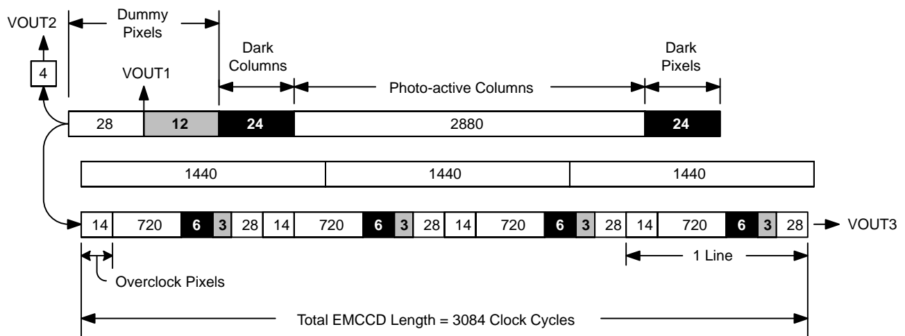
Figure 28. The Alignment of Pixels within the HCCD and EMCCD for 4x Horizontal Charge Binning when Transferring an Entire Line to the Left Side Outputs
